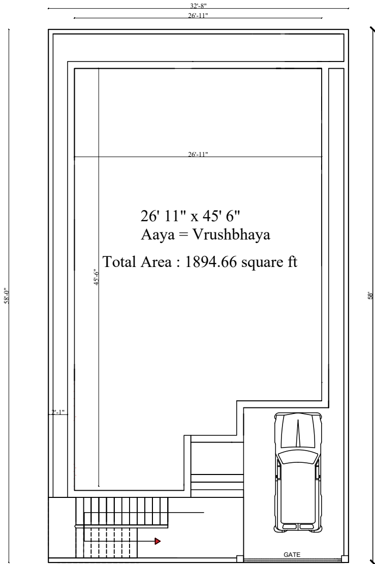
Site Plan
