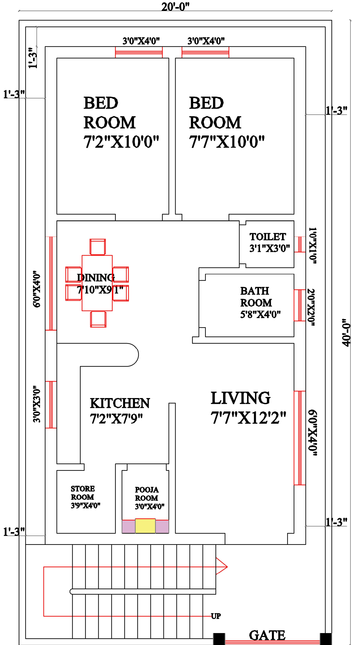
GROUND FLOOR
